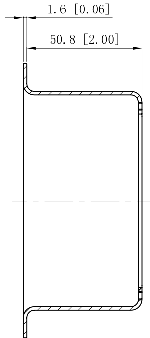
CUTAWAY VIEW A-A
