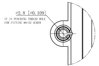
VIEW E
