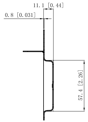
CUTAWAY VIEW A-A
