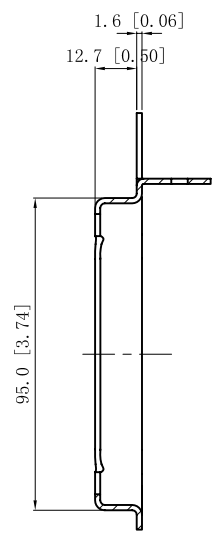
CUTAWAY VIEW A-A
