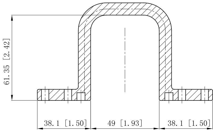
CUTAWAY VIEW A-A
