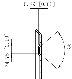
CUTAWAY VIEW A-A
